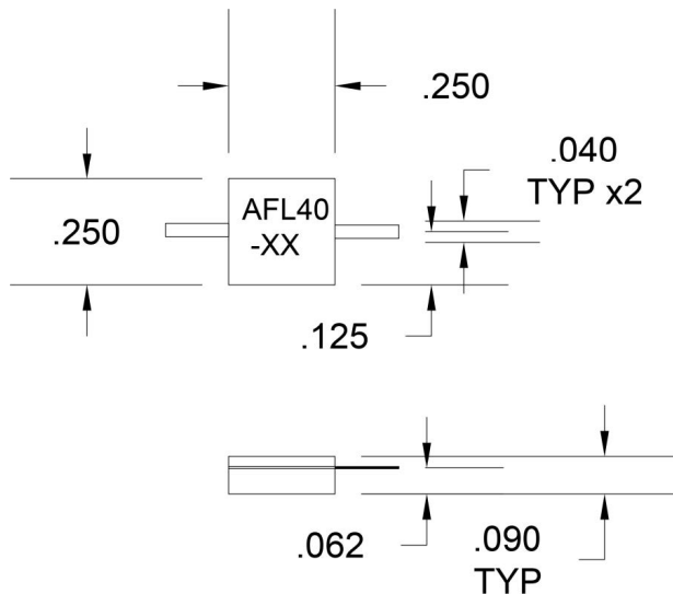
SUGGESTED MOUNTING AND TAB STRESS RELIEF METHOD
